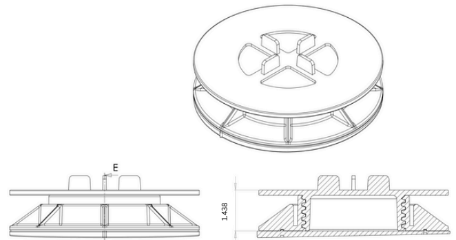
2 PIECE ADJUSTABLE PEDESTAL
