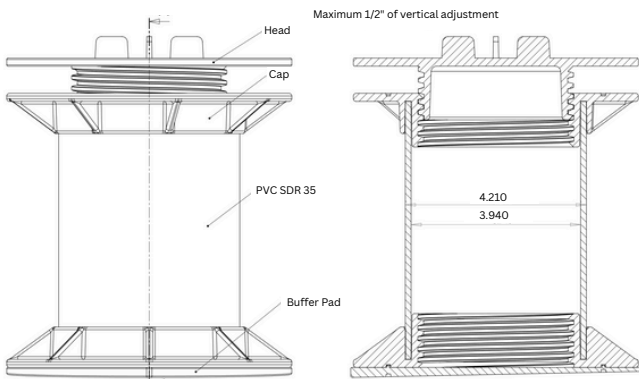
3 PIECE ADJUSTABLE PEDESTAL
