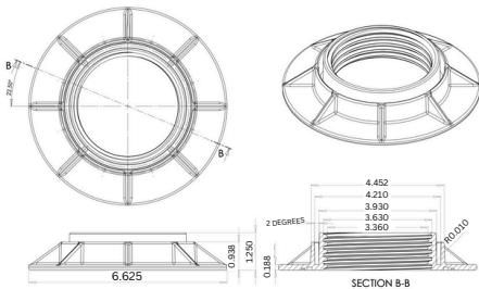
PEDESTAL END CAP
