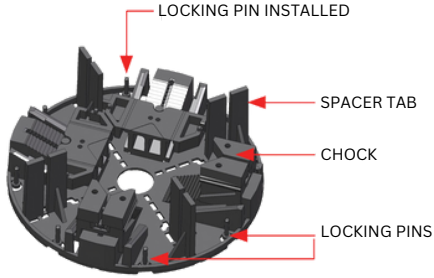
ONE STEP PEDESTAL
