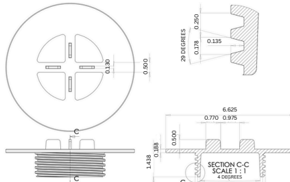
PEDESTAL TOP CAP
