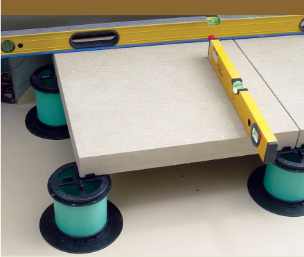
Concrete pavers over a PVC membrane
